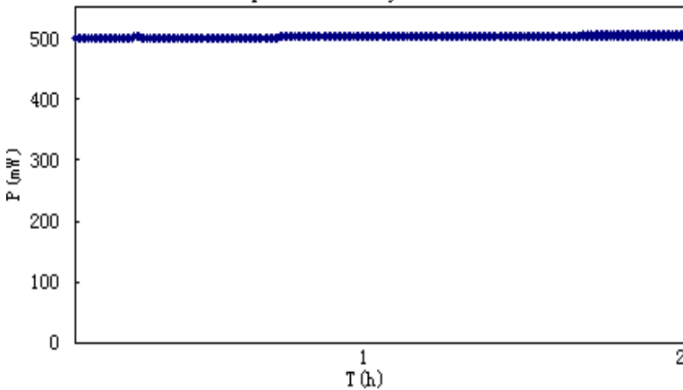
2hrs Power Stability of the GDL(Tc=25°C)
