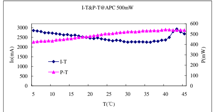
Current and Power vs. Temperature at APC Mode
