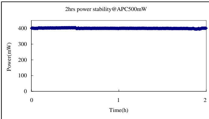
2hrs Power Stability of the GDL(Tc=25°C)
