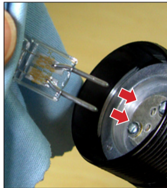
Align the 2 prongs of the replacement bulb with the 2 holes and insert.
